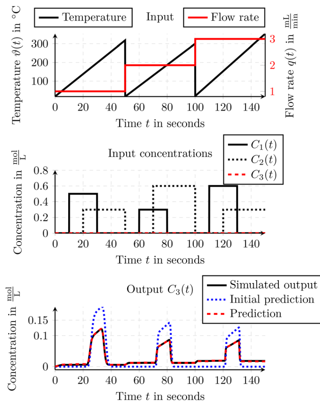
Fig. 8 Reactor simulation with flow-rate-depending offsets. Depicted is the output C_3(t) for the traditional tanks-in-series model, the initial prediction of the NTiS, and prediction of the trained NTiS.
