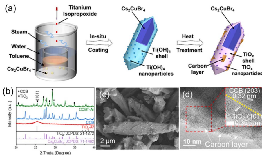
Fig. 6 (a) Schematic illustration of the synthesis procedure of CCBT-Ar catalysts. (b) XRD patterns of CCBT-Ar, CCB, and TiO x -Ar. (c) SEM image of CCBT-Ar. (d) High-resolution TEM image of CCBT-Ar (with a 5 nm bar size inset). Reproduced with permission from ref. 53. Copyright 2025, Elsevier.
