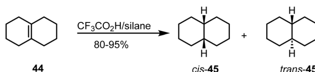
Scheme 17 Reduction of an exocyclic double bond.
