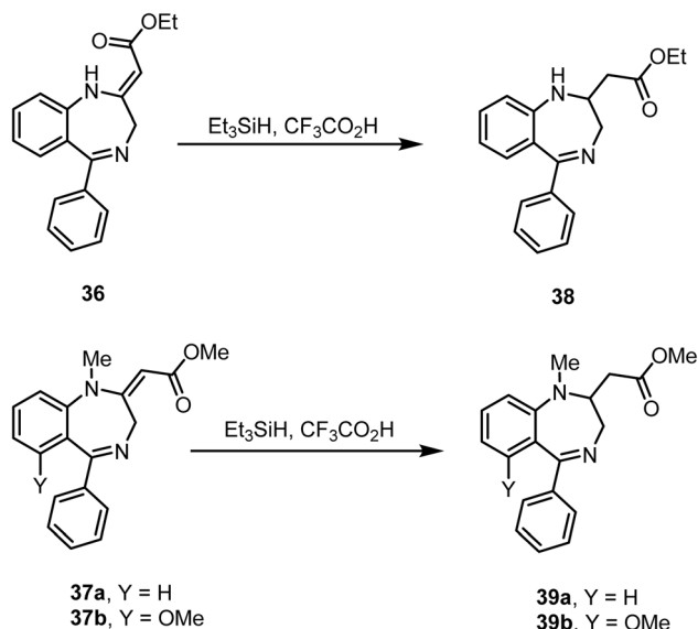
Scheme 15 Reduction of an exocyclic unsaturated ester.
