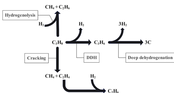
Fig. 1 Typical reaction pathways are often seen in the dehydrogenation of propane. In addition to the DDH process, there can also be cases of unwanted deep dehydrogenation causing coke formation, cracking, and hydrogenolysis. Adapted from ref. 3 with permission from the Royal Society of Chemistry, copyright 2021 (open access article under CC BY 3.0).
