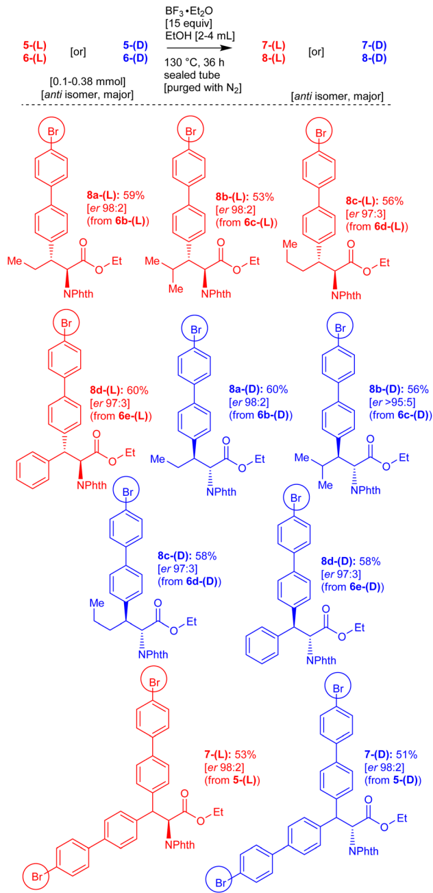
Scheme 6 Removal of the 8-aminoquinoline group and \text{BF}_3 \cdot \text{Et}_2\text{O} -mediated direct amide to ester conversion in substrates 5-(D), 6-(D), 5-(L) and 6-(L) affording the corresponding ester derivatives 7-(D), 8-(D), 7-(L) and 8-(L).
