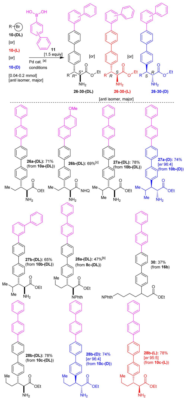
Scheme 12 Construction of quateraryl-based amino acid derivatives 26–30 via the Pd(II)-catalyzed Suzuki coupling reaction. Conditions: (a) \text{Pd}(\text{PPh}_3)_4 (5 mol%), \text{K}_2\text{CO}_3 (3 equiv.), toluene:EtOH:H 2 O (2:1:1 mL), 110 °C, 24 h, sealed tube (purged with N 2 ). (b) Compounds 28a-(DL) and 30 are obtained from 8c-(DL) and 16b using reaction conditions, \text{Pd}(\text{OAc})_2 (10 mol%), \text{P}(\text{o-tolyl})_3 (25 mol%), Et 3 N (0.2 mL), MeCN (3 mL), 85 °C, 17 h, sealed tube (purged with N 2 ). (c) Substrate 26b-(DL) was obtained from 10aa-(DL) . 18a
