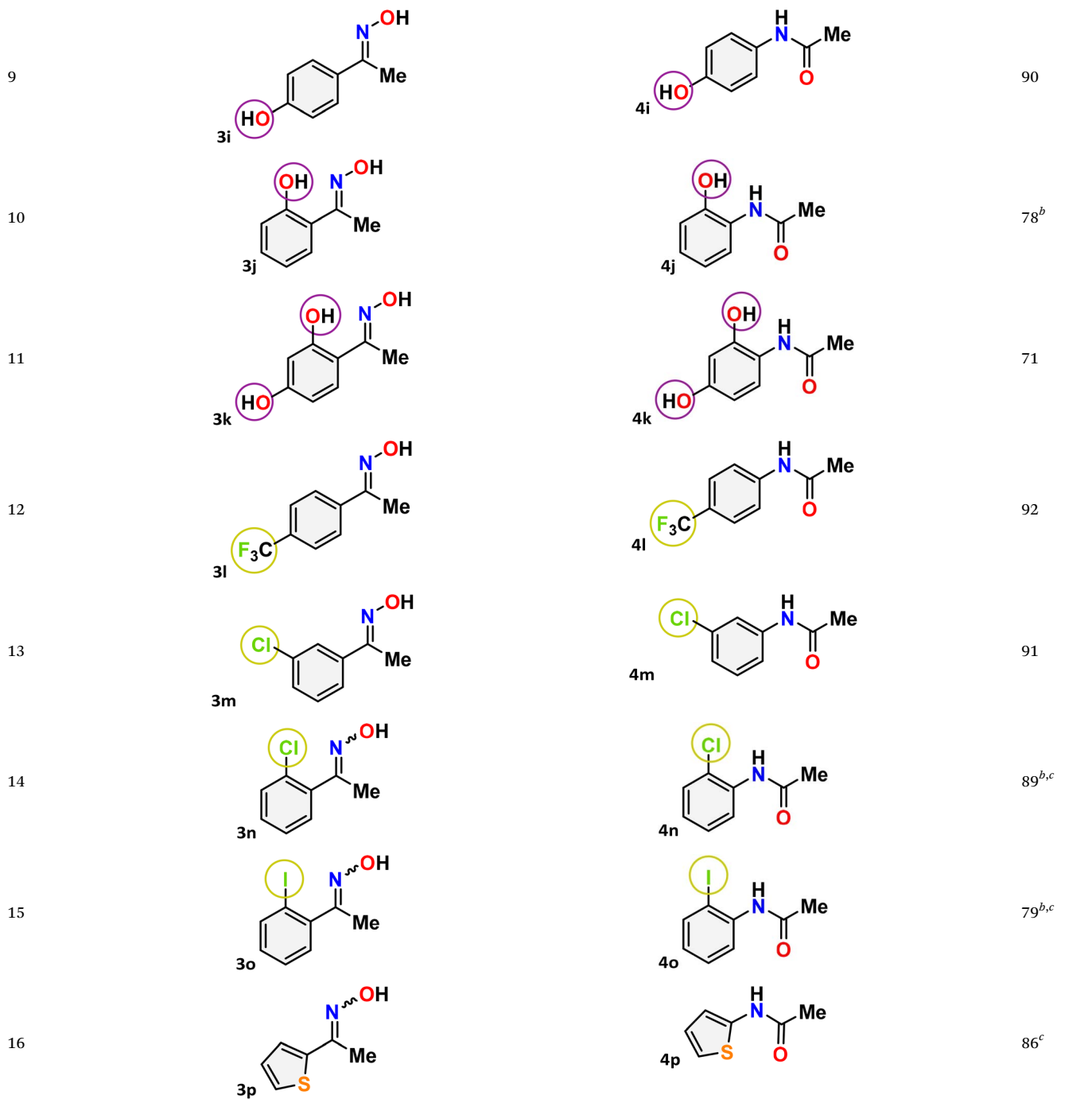
Entry Ketoximes Amides Yield (%)
