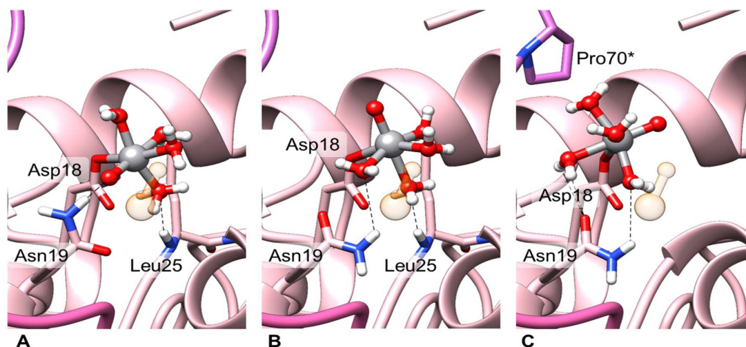
Fig. 13 Best covalent docking poses of [V^{IV}O]^{2+} at the symmetry mate-recreated binding site: (A) cluster I; (B) cluster II; (C) cluster III. The asterisk indicates the residue of HEWL symmetry mate chains (different shades of pink/purple). Hydrogen bonds are indicated with dashed lines. For comparison, the experimentally revealed VO group is reported in orange and in transparency with its crystallographic coordinates.
