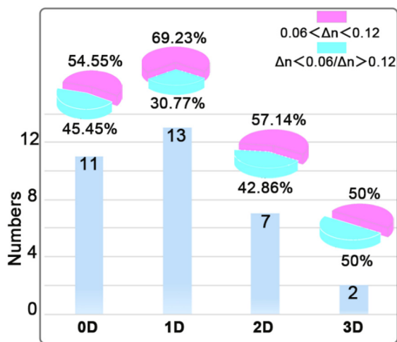
Fig. 4 Dimensional distribution statistics and birefringence distribution maps of the \text{SbOCl}\cdot\text{DMSO} with the most Sb-based oxygen containing acid salt NLO crystals in each dimension. All data are available in Table S5 in the ESI.†
