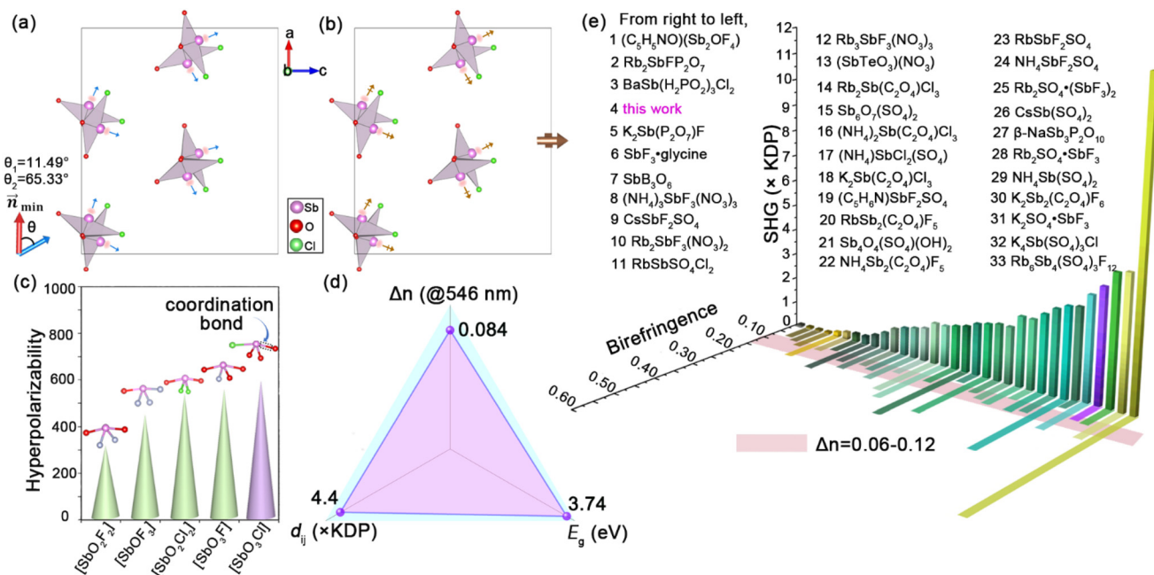
Fig. 5 (a) The angle diagram between the direction of lone pairs and the n_{\min} in \text{SbOCl}\cdot\text{DMSO} ; (b) the orientation of dipole moments in the unit cell for [\text{SbO}_3\text{Cl}]^{4-} groups in \text{SbOCl}\cdot\text{DMSO} , the direction of the overall dipole moments is highlighted by brown arrow; (c) comparison the hyperpolarizability of [\text{SbO}_2\text{F}_2] , [\text{SbOF}_3] , [\text{SbO}_2\text{Cl}_2] , [\text{SbO}_3\text{F}] , and [\text{SbO}_3\text{Cl}] ; (d) the radar plot of band gap E_g , SHG effect d_{ij} and \Delta n for \text{SbOCl}\cdot\text{DMSO} ; (e) the birefringence and SHG diagram for the \text{SbOCl}\cdot\text{DMSO} with the most Sb-based oxygen-containing acid salt NLO crystals. All data are available in Table S5 in the ESI.†
