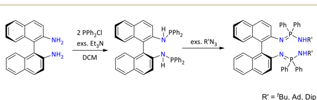
Scheme 58 Synthesis of C 2 -symmetric bis(iminophosphonamide) ligands. 33
