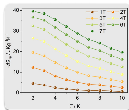
Fig. 2 Plot of experimental magnetic entropy change ( -\Delta S_m ) versus T for Gd 14 .
