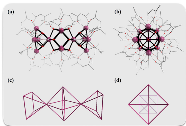
Fig. 1 (a) and (b) molecular structure, (c) and (d) metal core topology for Gd 14 . Color code: Gd (plum), O (red), C (grey). H atoms were omitted for clarity.
