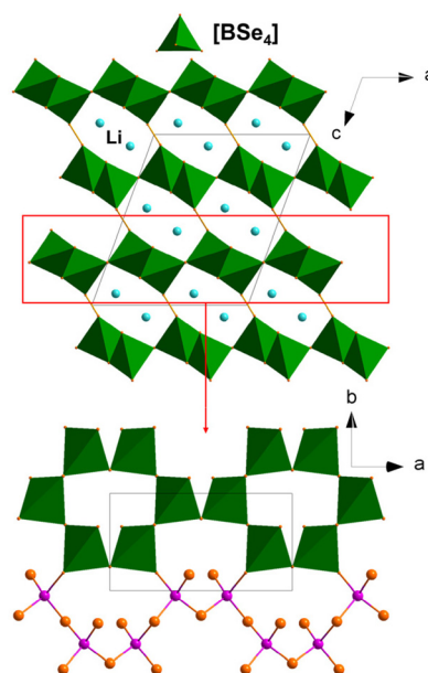
Fig. 11 The structure of \text{Li}_2\text{B}_2\text{Se}_5 .
