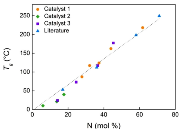
Fig. 4 Plot of glass transition temperature ( T_g ) vs. norbornene content in poly(P-co-N)s from Table 1 and the literature. 45 The dotted fitting line interpolates all the points on the graph.
