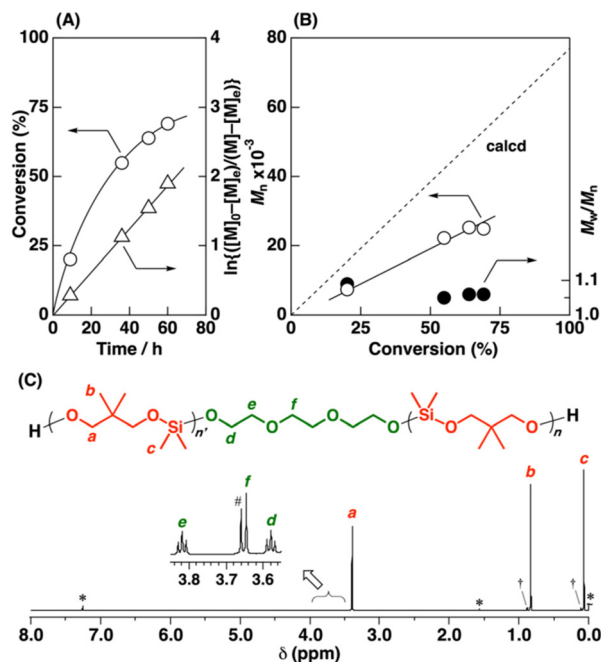
Fig. 1 (A) Time-conversion and first-order plots for the polymerization of Si6M, (B) the M n (open) and M w /M n (filled) values of poly(Si6M)s, and (C) 1 H NMR spectrum of poly(Si6M) (entry 1 in Table 1; in CDCl 3 at 30 °C; * Me 4 Si, water, or CHCl 3 ; # 13 C satellite; † very minor peaks observed near peaks b and c are not assigned yet). The data correspond to entry 1 in Table 1 (see Table 1 for the polymerization conditions).
