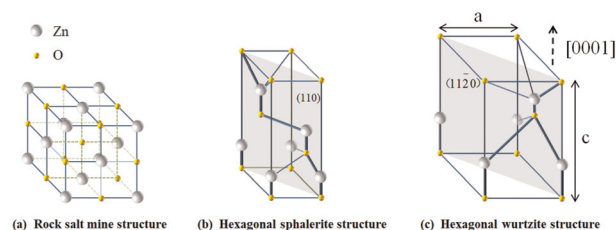
(a) Rock salt mine structure (b) Hexagonal sphalerite structure (c) Hexagonal wurtzite structure
