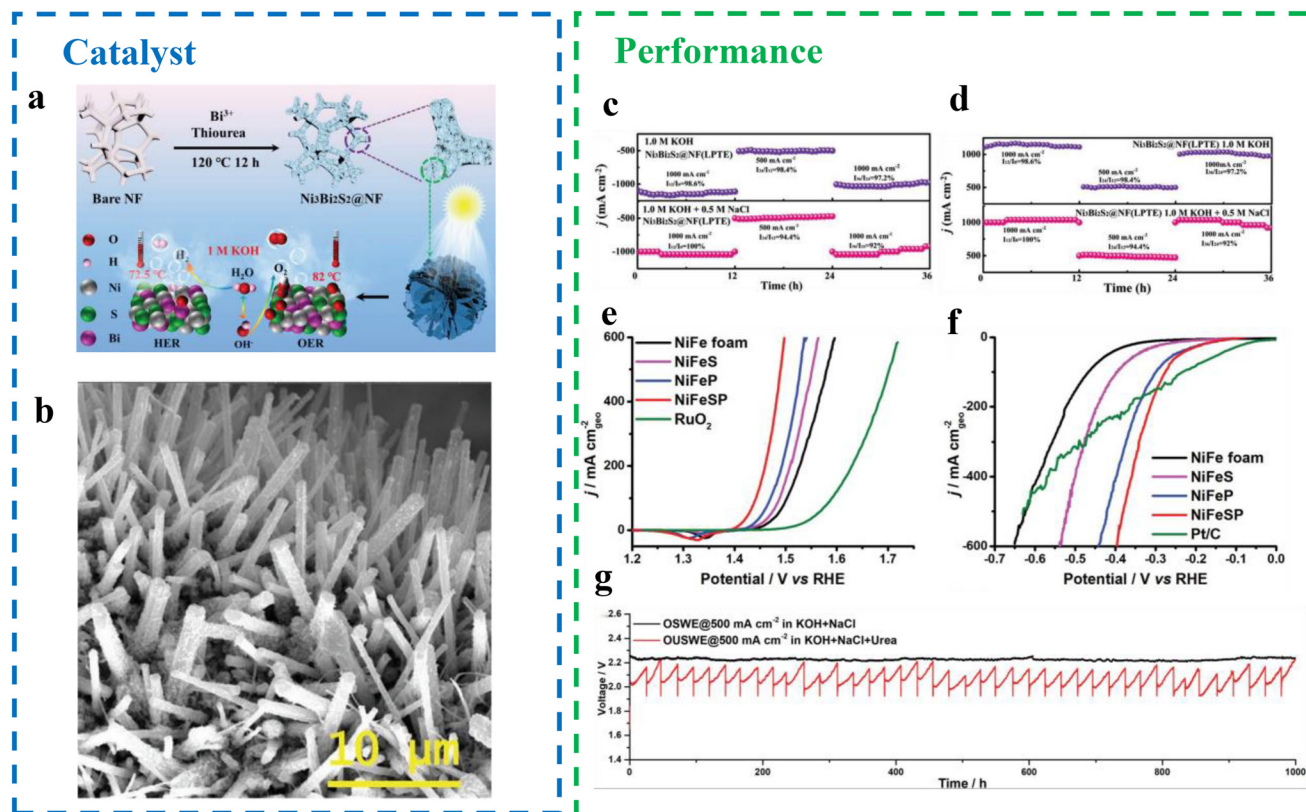
Fig. 18 (a) Illustration for preparing \text{Ni}_3\text{Bi}_2\text{S}_2@\text{NF} electrode and overall water splitting process with LPTE. 81 (b) SEM image of NiFeSP-NT. 82 (c) Long-time LPTE stability experiments of \text{Ni}_3\text{Bi}_2\text{S}_2@\text{NF} under different larger current density each for 12 h in 1.0 M KOH and simulated seawater solutions. 81 (d) Chronopotentiometric measurements of long-term stability of coupled-LPTE \text{Ni}_3\text{Bi}_2\text{S}_2@\text{NF} under different constant voltages for 12 h in 1.0 M KOH and 1.0 M KOH + 0.5 M NaCl solution. 81 Polarization curves of the (e) OER and (f) HER, recorded at 5 \text{mV s}^{-1} . 82 (g) Chronopotentiometric curves of the OSWE and OSUE for the NiFeSP electrode pair. 82
