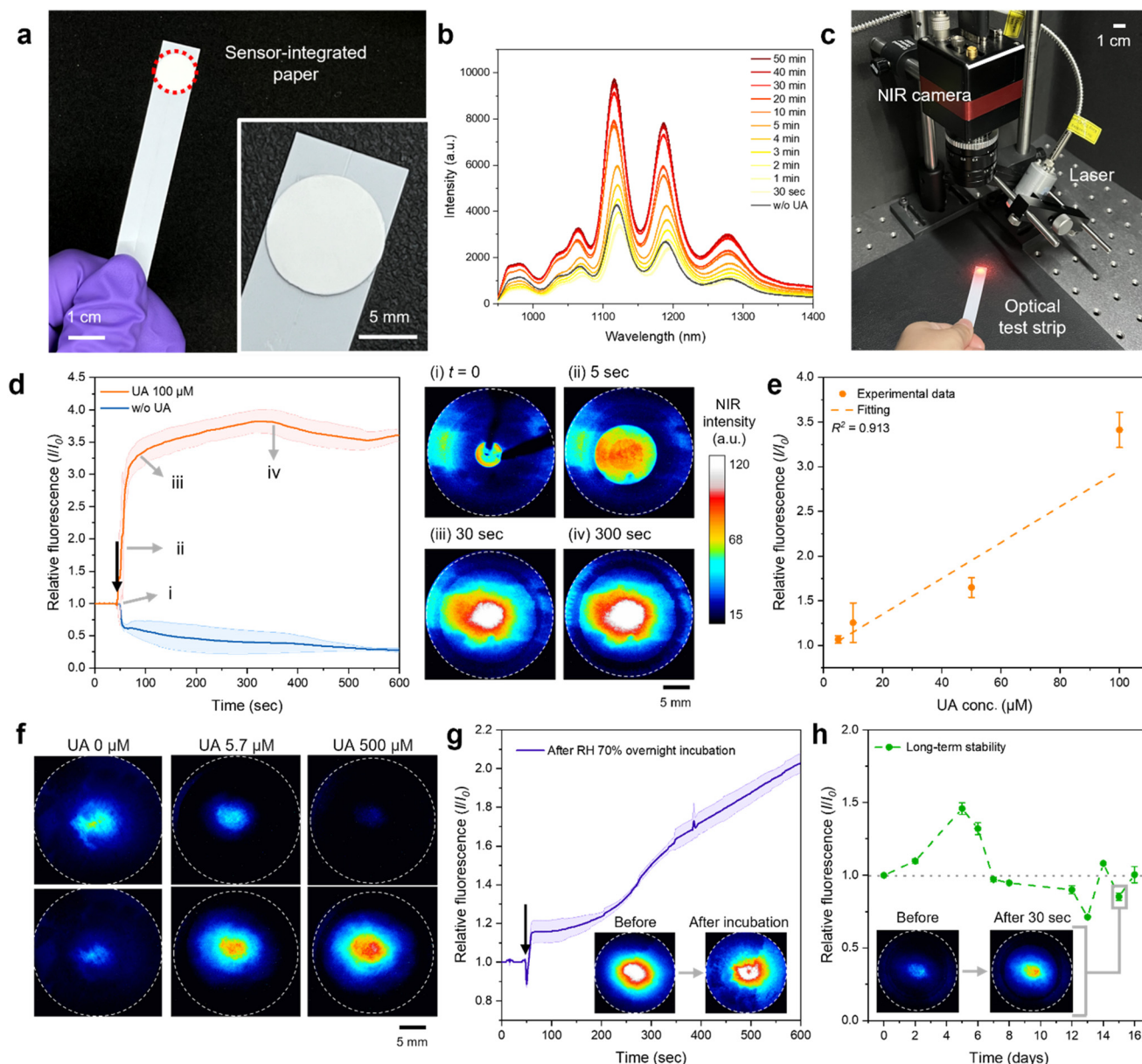
Fig. 4 Immobilization of the (\text{AAT})_{10}/\text{SWCNT} nanosensor on a paper substrate for POC UA monitoring. (a) Photograph of the optical test strip with corona nanosensor integration. (b) Real-time fluorescence variations of the corona nanosensor-integrated test strip following the addition of 100 \mu\text{M} UA in DI water. (c) Photograph of the onsite UA detection setup using a NIR camera. (d) Average fluorescence intensity profile of the corona nanosensor-integrated optical test strip following the addition of 100 \mu\text{M} UA in DI water at 50 s indicated by the black arrow, with the solid line representing the mean values and the shaded region indicating the standard deviation ( n = 3 ). The time-series NIR images (i–iv) correspond to the test strip marked in the profile, where the time denotes the elapsed period after the addition of UA solution. The region enclosed by the white dashed line represents the entire test strip area, and all images in this paper are presented using the same color scale. (e) Calibration curve of the corona nanosensor-integrated optical test strip with 5\text{--}100 \mu\text{M} UA in DI water ( n = 3 ). The relative fluorescence is defined as the ratio of the test strip's fluorescence intensity 1 minute after UA addition to its intensity before addition. (f) Captured images of the corona nanosensor-integrated test strip (upper) before and (lower) 30 s after the addition of DI water and 5.7 and 500 \mu\text{M} UA in human urine. (g) Average time profile of the fluorescence intensity of the optical test strip after dropping 100 \mu\text{M} UA in DI water at 50 s indicated by the black arrow, following incubation at 40^\circ\text{C} and 70\% RH overnight ( n = 3 ). The inset images show the baseline NIR signals before and after incubation. (h) Stably preserved NIR fluorescence intensity of the test strip for 16 days ( n = 3 ). The inset images show test strip response to 100 \mu\text{M} UA in DI water after 15 days of storage.
