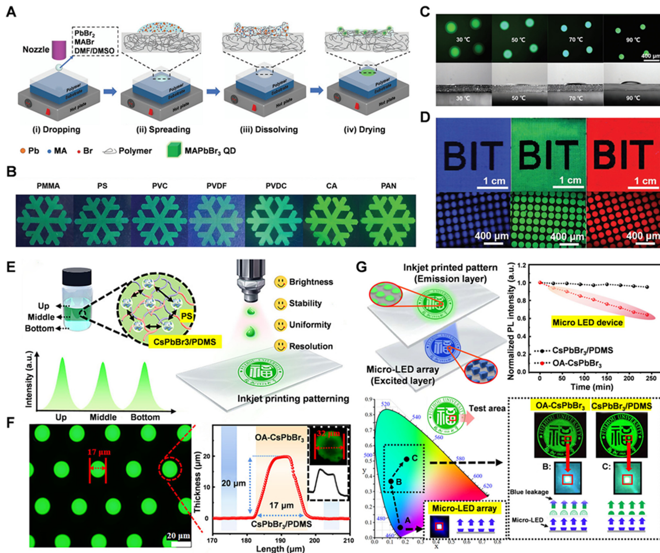
Fig. 5 (A) Schematic of the piezoelectric inkjet printing of the perovskite precursor solution droplet on the polymer-coated substrate and the crystallization after. (B) Formed perovskite patterns on different polymer substrates. (C) Photograph of perovskite microdisks and contact angle of the precursor solution on the PAN substrate at a temperature of 30 °C–90 °C. (D) Blue-, green- and red-perovskite QD arrays. Reprinted with permission from ref. 25. Copyright 2019, John Wiley and Sons. (E) Schematic of the piezoelectric inkjet printing of for creating color conversion pattern. (F) Fluorescent image of the printed PDMS-encapsulated CsPbBr 3 QD arrays and the corresponding size profile. (G) Schematic of the color conversion layer with blue micro-LED excitation, and the comparison of PL intensity and blue light leakage of PDMS-encapsulated CsPbBr 3 QDs and the control sample OA-CsPbBr 3 QD. Reprinted with permission from ref. 26. Copyright 2024, John Wiley and Sons.
