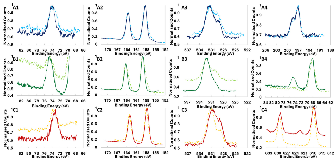
Fig. 5 High resolution XPS curves of: (A) BiOCl, (B) BiOBr and (C) BiOI coated with 1 cycle of ALD at 60 °C. Traces corresponding to Al, Bi, O and X (Cl, Br or I) atoms are denoted by indexes 1–4, respectively. Continuous curves represent samples coated following UVOC pretreatment, while dashed curves represent samples coated without UVOC pretreatment.
