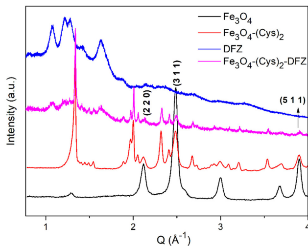
Fig. 8 X-ray powder diffraction patterns of \text{Fe}_3\text{O}_4 (black line), \text{Fe}_3\text{O}_4 -(Cys) 2 (red line), \text{Fe}_3\text{O}_4 -(Cys) 2 -DFZ (magenta line) and DFZ (blue line). The diffractograms were normalized by the maximum peak intensity and vertically displaced for better visualization.
