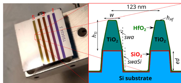
Fig. 1 On the left, a picture of the sample wafer is shown with the five different sample stripes visible. Stripe 1 denotes the unetched sample, while 3 marks the lesser etched and 5 the greater etched grating structure. On the right, a schematic cross section of the \text{TiO}_2 gratings with the parameters defining the sample model is shown. Only two of the approximately 8000 grating lines in the 1 mm wide stripe are shown. The sample model consists of a Si substrate with a \text{SiO}_2 top layer. On top of this a \text{TiO}_2 layer is located. A grating structure is etched into the layered sample, the grating lines may protrude into the Si substrate. The resulting structure is then covered by a \text{HfO}_2 layer. The etching depth varies between the different sample stripes.
