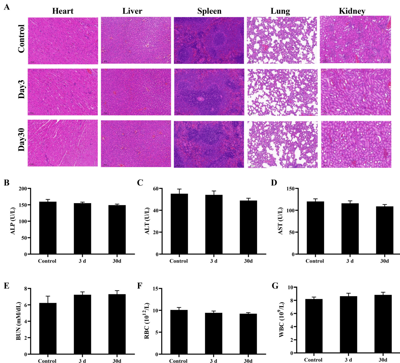
Fig. 9 H&E staining of major organs, scale bar: 100 μm (A). Blood analysis of the liver and kidney indicators (B–G).
