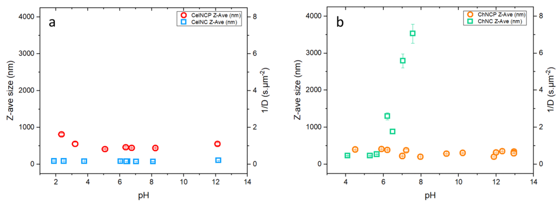
Fig. 3 Dimensions (equivalent sphere diameter) and inverse diffusion coefficient ( 1/D ) for polysaccharide cellulose and chitin nanocrystals dispersed in aqueous medium at different \text{pH} : (a) pristine and phosphorylated cellulose nanocrystals (CellNC, CellNC-P); (b) pristine and phosphorylated chitin nanocrystals (ChitNC, ChitNC-P). For most samples, the error bars displayed in the figure are smaller than the symbols size.
