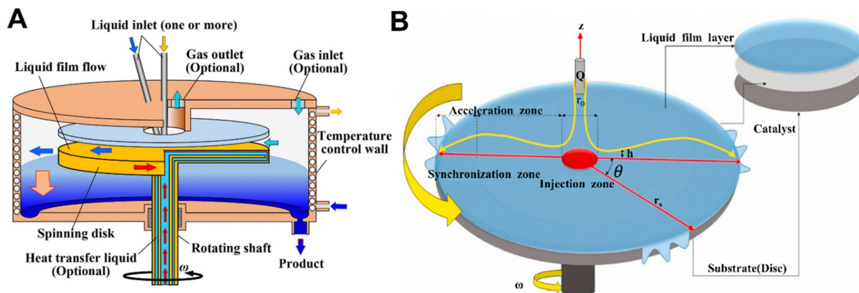
Fig. 6 (A) Schematic diagram of the basic components and operating principle of the SDR. Adapted with permission from ref. 88. Copyright 2023 Elsevier. 88 (B) Location of the injection, acceleration and synchronization zones on the disk. Adapted with permission from ref. 89. Copyright 2024 Elsevier. 89
