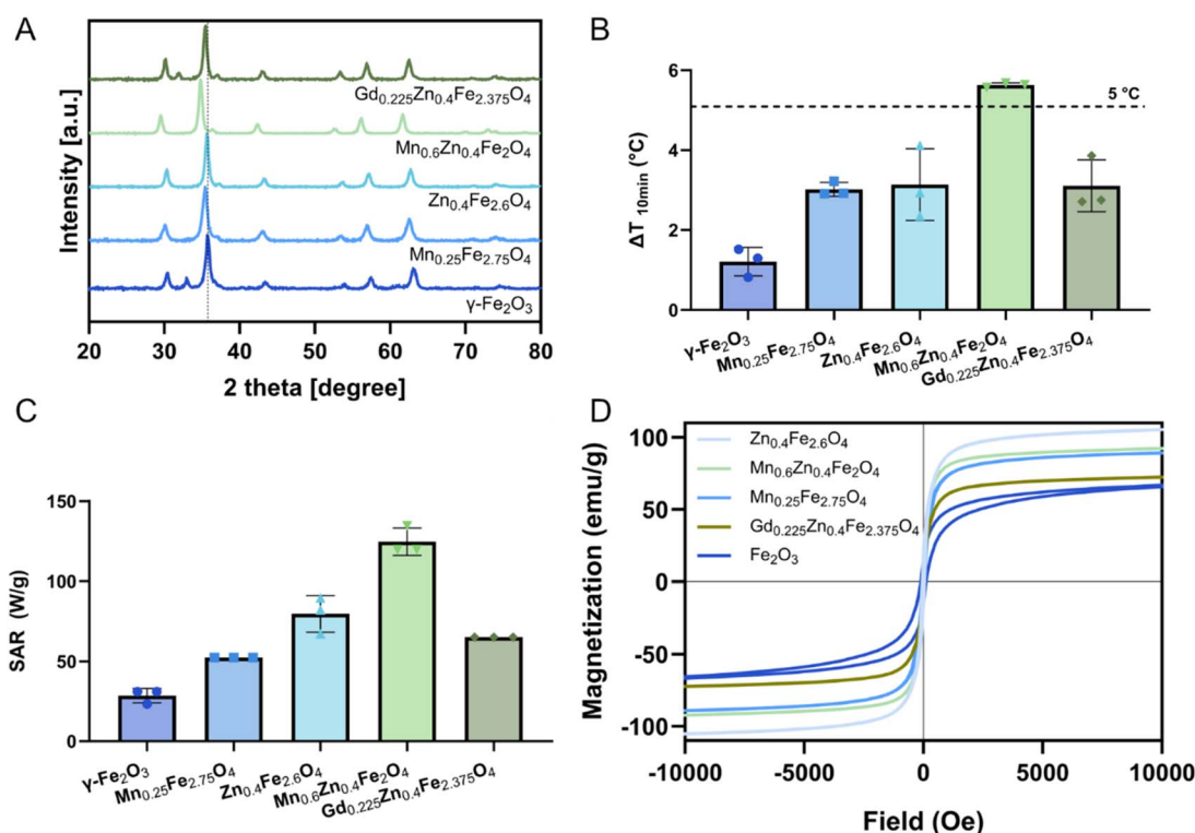
Fig. 2 Characterization of silica-coated SPIONs with different core compositions. (A) XRD pattern of silica-coated \gamma\text{-Fe}_2\text{O}_3 , \text{Mn}_{0.25}\text{Fe}_{2.75}\text{O}_4 , \text{Zn}_{0.4}\text{Fe}_{2.6}\text{O}_4 , \text{Mn}_{0.6}\text{Zn}_{0.4}\text{Fe}_2\text{O}_4 and \text{Gd}_{0.225}\text{Zn}_{0.4}\text{Fe}_{2.375}\text{O}_4 . The dashed line marks the (311) plane of the maghemite crystal structure. (B) Temperature change ( \Delta T ), and (C) specific absorption rate (SAR) of silica-coated doped ferrites in water suspension after 10 min of AMF exposure ( f = 592.3 \text{ kHz} , H = 14 \text{ mT} ). Data are expressed as mean \pm SD ( n = 3 ). The dashed line in (B) represents \Delta T = 5^\circ\text{C} , the temperature increase commonly recommended for hyperthermia treatment. (D) Magnetic field dependence of magnetization at 27^\circ\text{C} of silica-coated \gamma\text{-Fe}_2\text{O}_3 , \text{Mn}_{0.25}\text{Fe}_{2.75}\text{O}_4 , \text{Zn}_{0.4}\text{Fe}_{2.6}\text{O}_4 , \text{Mn}_{0.6}\text{Zn}_{0.4}\text{Fe}_2\text{O}_4 and \text{Gd}_{0.225}\text{Zn}_{0.4}\text{Fe}_{2.375}\text{O}_4 .
