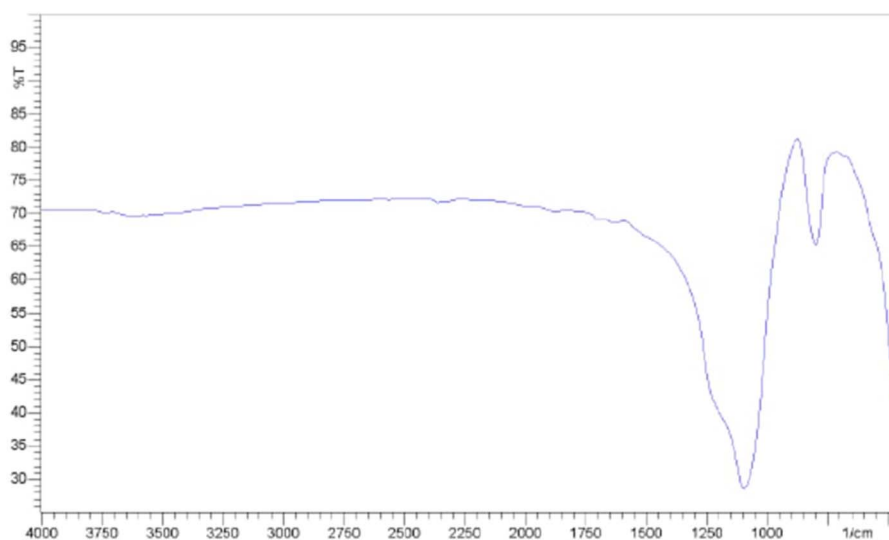
Fig. 5 FTIR spectra of silica. 38,41,42
