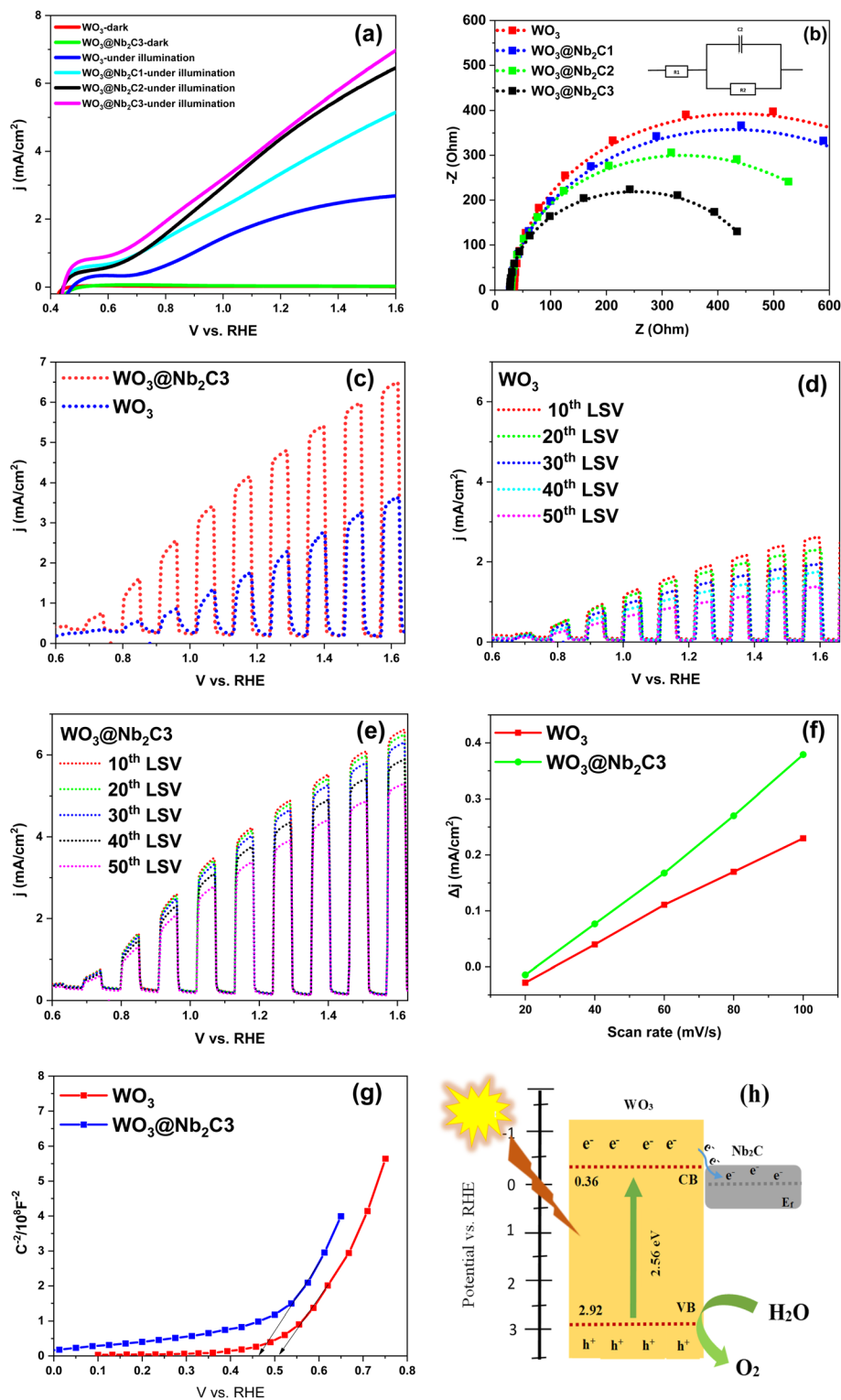
Fig. 7 PEC activities of pure \text{WO}_3 and \text{WO}_3/\text{Nb}_2\text{CT}_x in 0.5 \text{ M Na}_2\text{SO}_4 : (a) LSV curves, (b) Nyquist plots, (c) chopped light LSV curves, (d) chopped light LSV curves for cyclic stability for \text{WO}_3 , (e) chopped light LSV curves for cyclic stability for \text{WO}_3/\text{Nb}_2\text{C}_3 composite, (f) double layer capacitance plots for \text{WO}_3/\text{Nb}_2\text{C}_3 composite, (g) Mott-Schottky plots for \text{WO}_3 and \text{WO}_3/\text{Nb}_2\text{C}_3 composite, and (h) charge carrier generation/separation and participation in water splitting.
