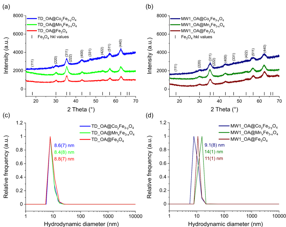
Fig. 1 PXRD diffraction patterns of the particles synthesized with (a) TD method and (b) MW1 method in comparison with the \text{Fe}_3\text{O}_4 reference structure 50 and their respective DLS measurements (c) and (d) measured in n -hexane.
