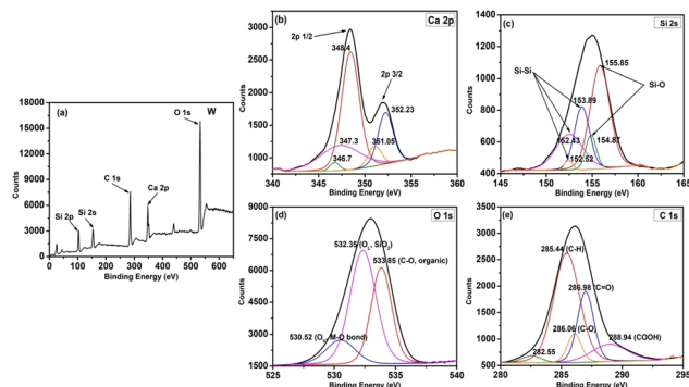
Fig. 1 XPS data for pristine wollastonite ( \text{CaSiO}_3 ), including (a) full survey and (b–e) high-resolution images of individual components.
