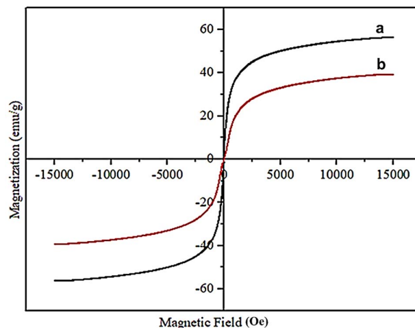
Fig. 7 VSM of (a) \text{Fe}_3\text{O}_4 and (b) \text{Fe}_3\text{O}_4\text{@C@TiO}_2/\text{melamine} .
