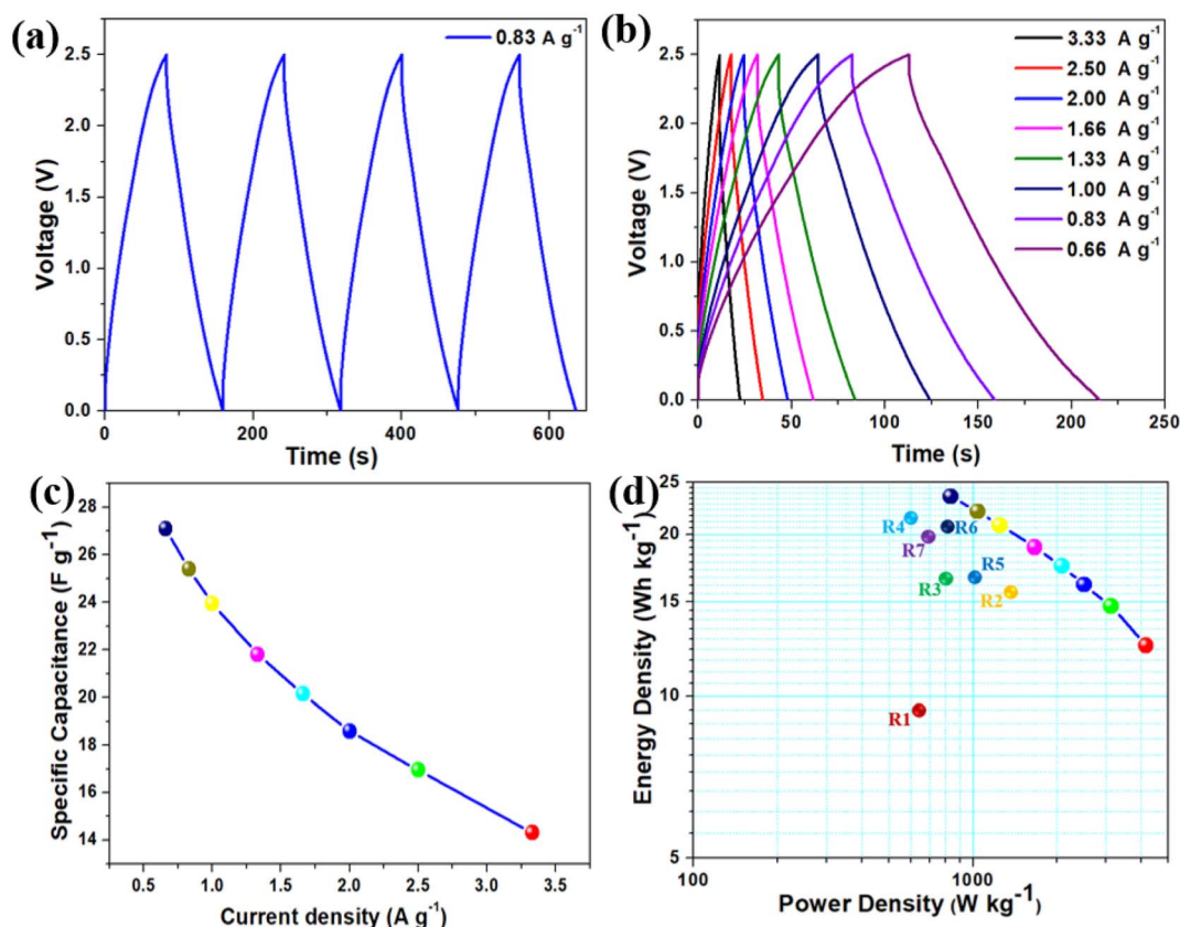
Fig. 6 (a) The galvanostatic charge–discharge profiles of BAC-based SCSD measured at a constant current of 0.83\ \text{A g}^{-1} in the operating potential window from 0.0 to 2.5\ \text{V} . (b) Charge–discharge profiles of BAC-based SCSD recorded in different applied current ranges from 3.33 to 0.66\ \text{A g}^{-1} . (c) The effect of discharge current on the gravimetric specific capacitance of BAC-based SCSD. (d) a Ragone plot showcasing the performance metrics of BAC-based SCSD highlights their superior capabilities compared to previously reported supercapacitors utilizing ionic liquid electrolytes. The references (R1–R7) in Fig. 4(D) are provided in Table S3 (in ESI).†
