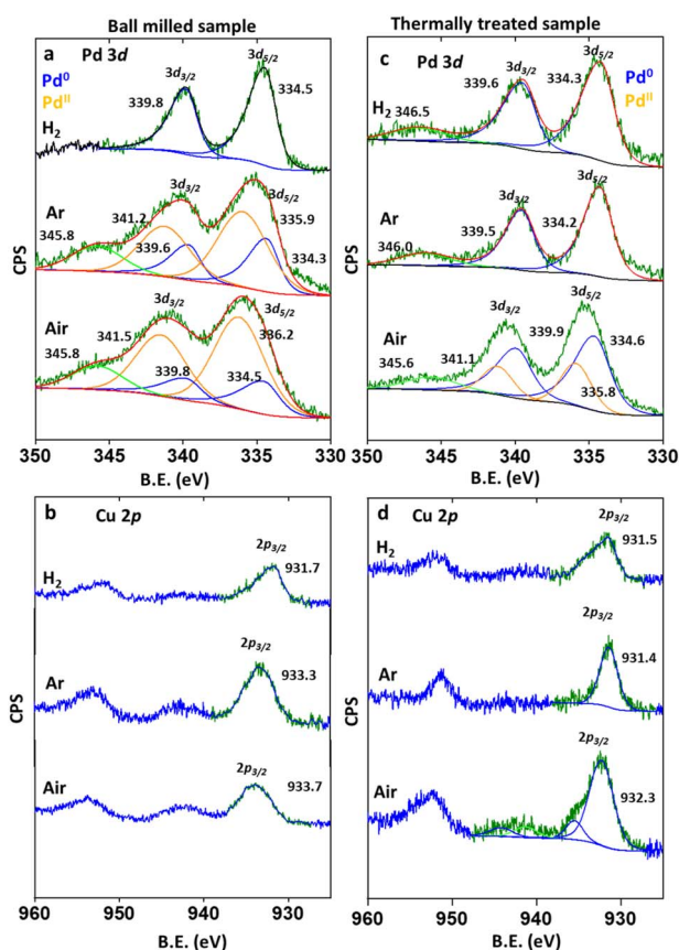
Fig. 4 XPS spectra of 5 wt% Pd 1 Cu 1 /α-Al 2 O 3 after ball milling in oxidative (air), inert (Ar), reductive (H 2 ) atmospheres for Pd 3d (a) Cu 2p (b), and XPS spectra for these samples after thermal treatment for Pd 3d (c) Cu 2p (d).
