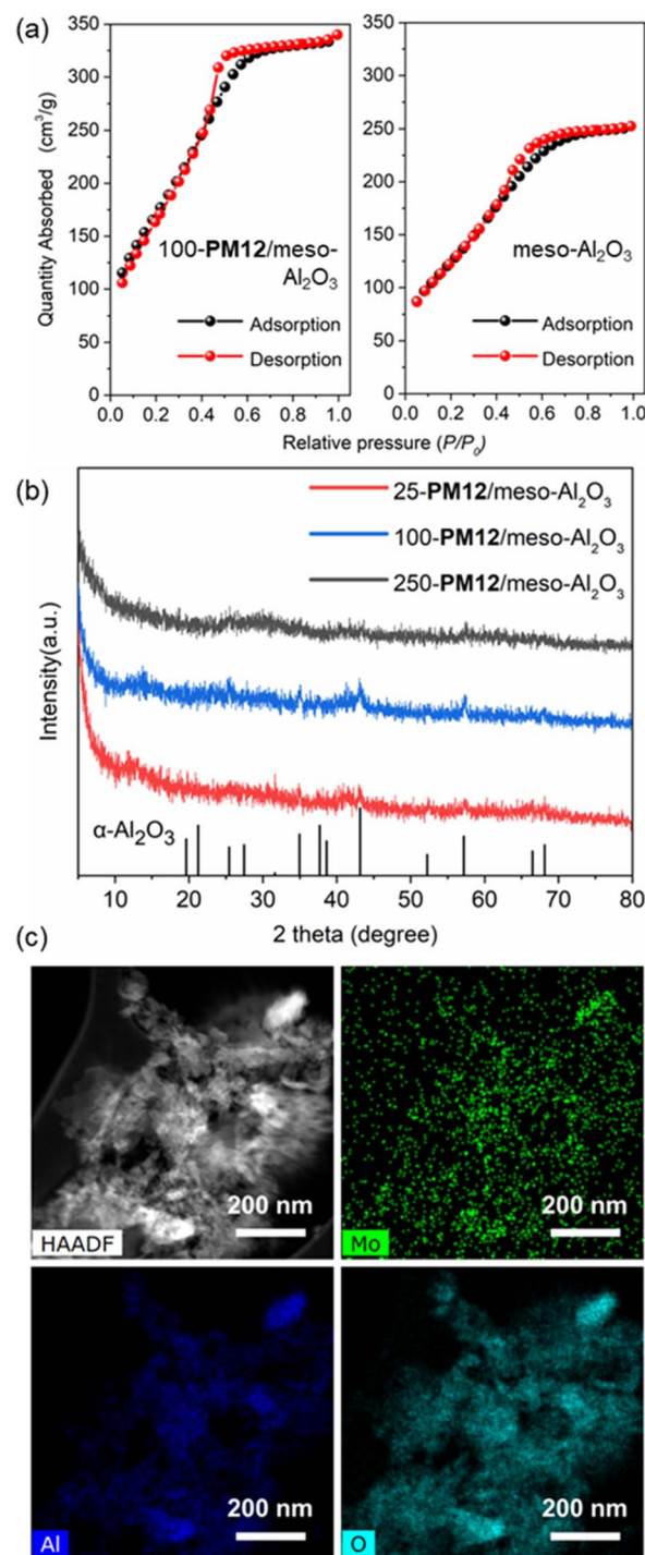
Fig. 2 (a) N 2 adsorption-desorption isotherms (77 K) of 100- PM12 /meso- \text{Al}_2\text{O}_3 and meso- \text{Al}_2\text{O}_3 ; (b) XRD spectra of varying loading amounts of POMs as x\text{-PM12/meso-Al}_2\text{O}_3 ; (c) STEM EDS-mapping images of 100- PM12 /meso- \text{Al}_2\text{O}_3 .
