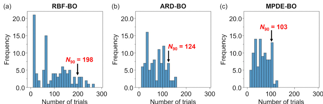
Fig. 2 Number of trials required to determine the global maximum of the model function of (d, s) = (3, 1) using (a) RBF-BO, (b) ARD-BO, and (c) MPDE-BO, where d and s represent the number of important and unimportant synthesis parameters, respectively. RBF-BO, ARD-BO, and MPDE-BO correspond to Bayesian optimization (BO) using RBF kernel, BO using ARD kernel for sparse estimation, and BO using MPDE kernel for sparse estimation, respectively. Each histogram was obtained using 100 model functions with the same value of P_w but different peak positions.
