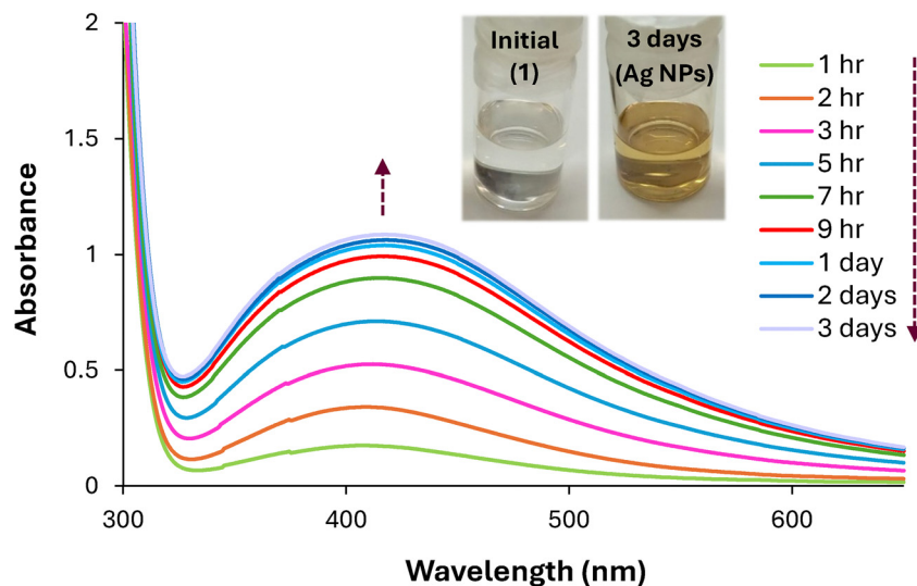
Fig. 19 Electronic spectral changes as a function of time during the formation of silver NPs by the IMR reaction of the Ag I complex ( 1 ) in methanolic solution (417 \mu\text{M} ).
