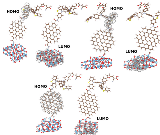
Fig. 6 Isocontour of the HOMO and LUMO densities for the \text{WD8@C42@TiO}_2 , \text{WD8@C54@TiO}_2 and \text{WD8@C66@TiO}_2 systems with CAM-B3LYP. The isocontour value is chosen as 0.01a_0^{-3} .
