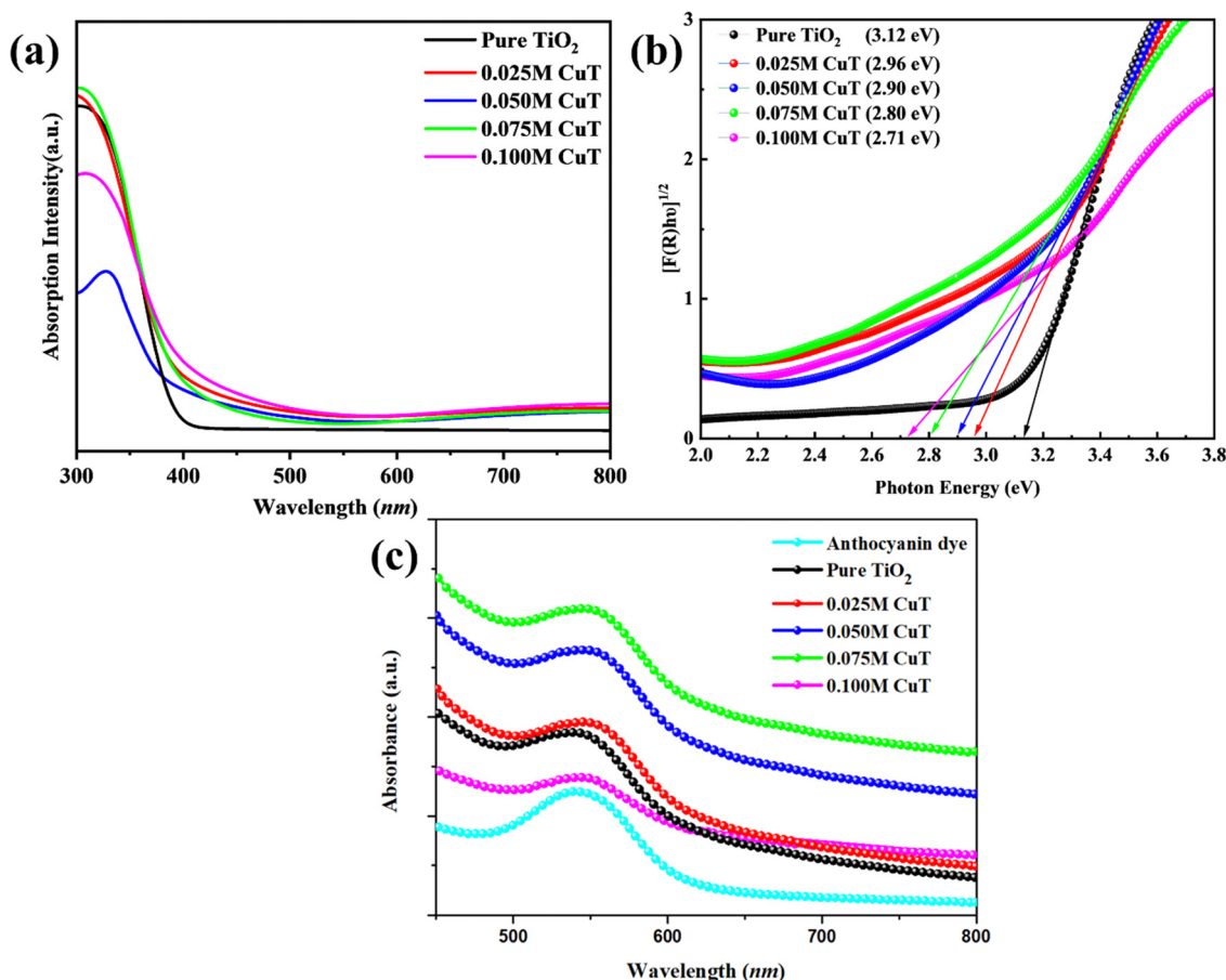
Fig. 7 (a) and (b) UV-Vis absorbance spectra and Tauc plots for undoped TiO 2 and different Cu-doped TiO 2 samples; and (c) absorbance spectra of anthocyanin sensitized various TiO 2 films.
