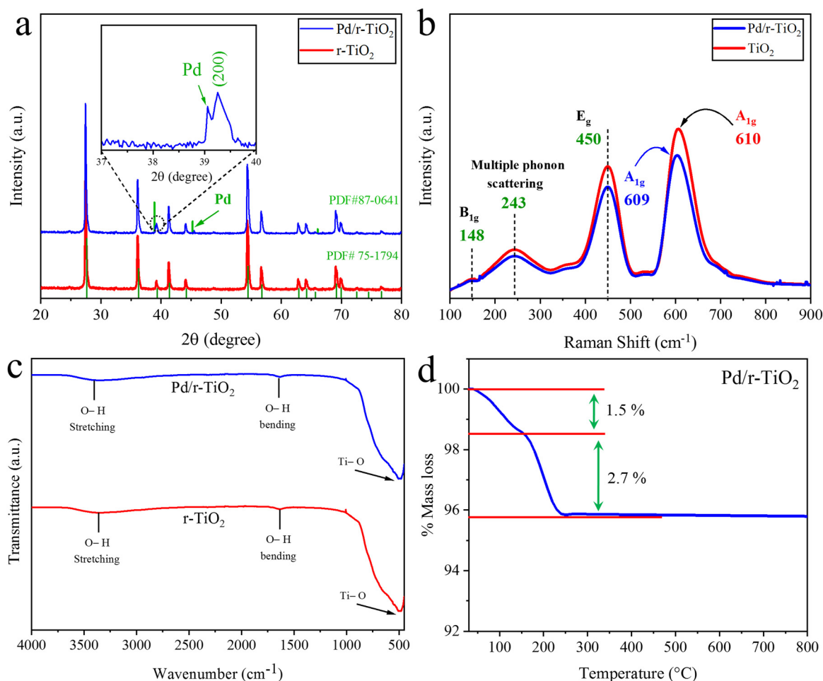
Fig. 2 (a) XRD patterns (inset: zoomed view of Pd diffraction), (b) Raman spectrum, (c) FTIR results r\text{-TiO}_2 and Pd/ r\text{-TiO}_2 and (d) TGA analysis of Pd/ r\text{-TiO}_2 .
