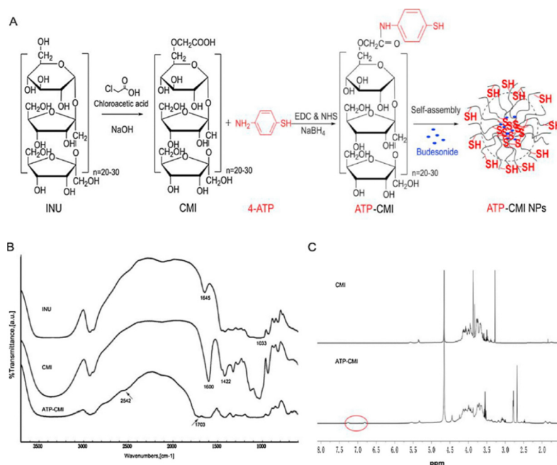
Fig. 9 (A) Synthetic procedure of CMI, ATP-CMI conjugate and ATP-CMI NPs. (B) FT-IR spectra of INU, CMI, and ATP-CMI conjugate. (C) 1 H NMR spectra of CMI and ATP-CMI conjugate in D 2 O. Reprinted from Q. Sun, L. Luan and M. Arif et al. , Redox-sensitive nanoparticles based on 4-aminothiophenol-carboxymethyl inulin conjugate for budesonide delivery in inflammatory bowel diseases, Carbohydr. Polym. , 189 , 352–359, Copyright (2018), with permission from Elsevier.
