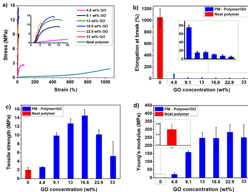
Fig. 5 Mechanical testing of P(BzMA- stat -nBA)/GO nanocomposite films containing different concentrations of GO for physical mixing systems; (a) stress-strain curves; (b) elongation at break; (c) tensile strength; (d) Young's modulus.
