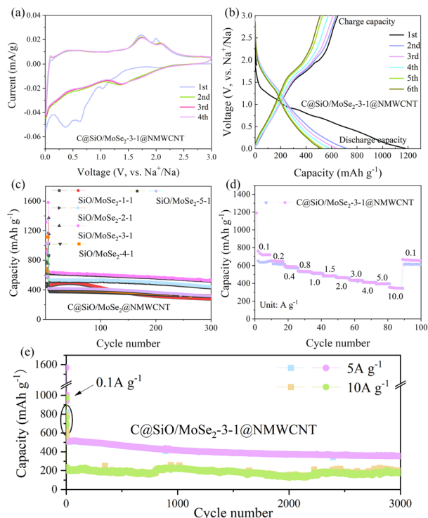
Fig. 5 (a) CV curves at a scan rate of 0.1 \text{ mV s}^{-1} , (b) galvanostatic discharge and charge voltage curves ( 0.1 \text{ A g}^{-1} ) of \text{C@SiO}_x/\text{MoSe}_2\text{-3:1@NMWCNT} , (c) discharge and charge profiles ( 0.5 \text{ A g}^{-1} ) of \text{C@SiO}_x/\text{MoSe}_2\text{-1/2/3/4/5:1@NMWCNT} , (d) rate capacity of \text{C@SiO}_x/\text{MoSe}_2\text{-3:1@NMWCNT} , (e) long-term tests ( 5 \text{ A g}^{-1} , 10 \text{ A g}^{-1} ) of \text{C@SiO}_x/\text{MoSe}_2\text{-3:1@NMWCNT} .
