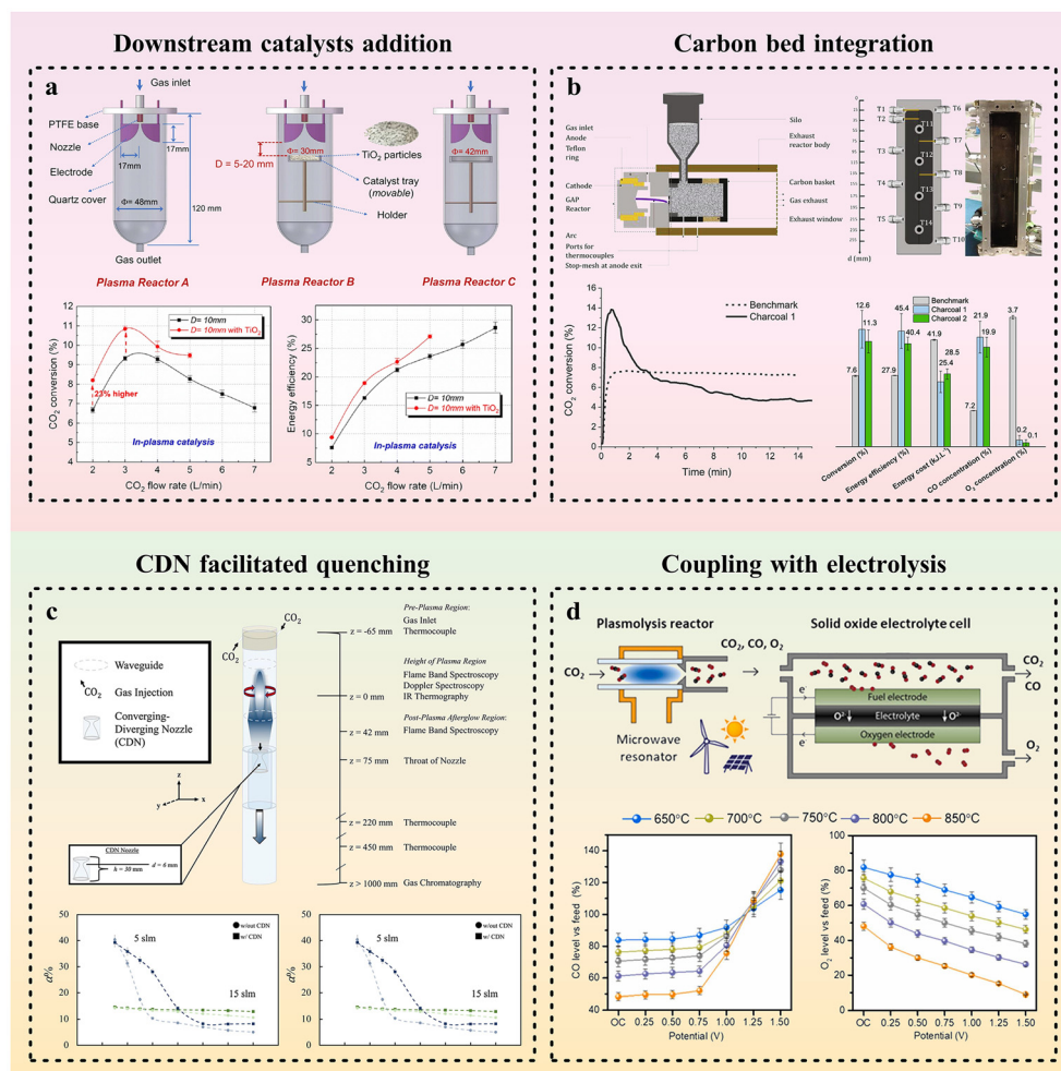
Fig. 5 Post-plasma techniques for \text{CO}_2 dissociation in GAD and MWD plasma systems. (a) Downstream catalyst addition. Reproduced from ref. 137 with permission from Springer Nature, copyright 2020. (b) Carbon bed integration in GAD plasma systems. Reproduced from ref. 125 with permission from Elsevier, copyright 2022. (c) Converging-diverging nozzle facilitated quenching. Reproduced from ref. 109 with permission from Elsevier, copyright 2023. (d) The coupling with electrolysis in MWD plasma systems. Reproduced from ref. 70 with permission from Elsevier, copyright 2022.
