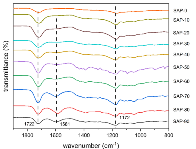
Fig. 4 FTIR spectra of extracted SAPs synthesized from CA, MSC, and GLY and after thermal cross-linking. Molar feed ratio of (CA + MSC)/GLY is always 1/1, weighed in molar monomer ratios CA/MS (ND) indicated in the figure.
