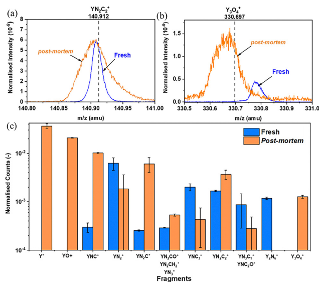
Fig. 5 ToF-SIMS Y-based fragments before (fresh) and after ( post-mortem ) electrochemical testing of CNGO-0.50 Y in positive SIMS spectrum shown for (a) YN_2C_2^+ , (b) Y_3O_4^+ , and (c) list of identified major fragments. Fragment counts from peak areas were normalized to the total ion counts.
