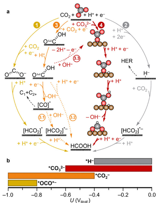
Fig. 16 (a) Reaction network of e\text{CO}_2\text{RR} and carbonate reduction mechanisms leading to HCOOH. The consensual e\text{CO}_2\text{RR} mechanisms to formate start by \eta_{\text{O,O}}^* \text{OCO}^- (path 1) or by ^*\text{H}^- (path 2) adsorptions. Additionally, path 3 leads to ^*\text{CO} which can further evolve to HCOOH by hydration (path 3.1). ^*\text{COOH} can also evolve to HCOOH (path 3.2). Path 4 is the newly proposed carbonate mechanism that can have contributions from path 3 through the conversion of the ^*\text{COOH} intermediate (path 3.3). (b) Range of potential stability of different intermediates. 116 Reproduced with permission from ref. 116, copyright 2023 American Chemical Society.
