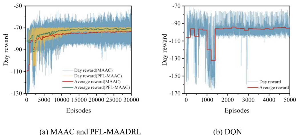
Fig. 2 Algorithm convergence curves. (a) MAAC and PFL-MAADRL, (b) DQN.
