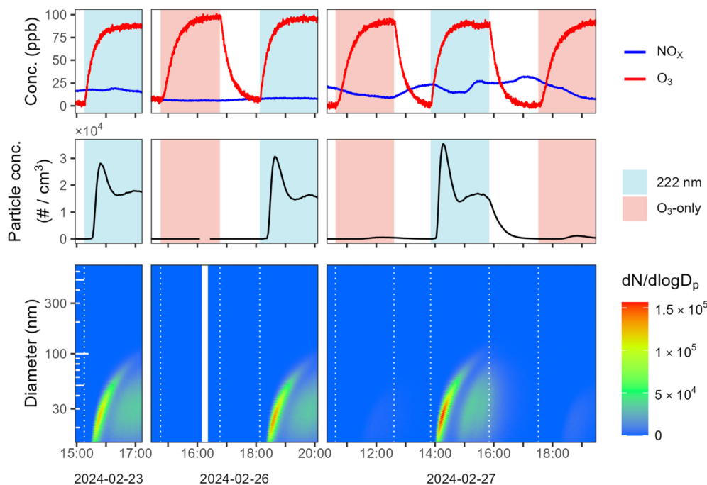
Fig. 2 New particle formation for experiments using sampled outdoor air. Shown are \text{O}_3 and \text{NO}_x concentrations over time (top row), particle number concentration over time (second row) for six experiments in which outdoor air is introduced (expts 35–40). Experiments are carried out on three separate days. The 222 nm lamp is turned on, and when the ozone generator is turned on, are highlighted in pale blue and pale red, respectively, in the top two rows.
