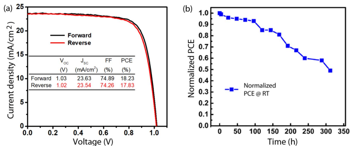
Fig. 6 Photovoltaic performance of the champion perovskite solar cells. (a) Current density vs. voltage ( J-V ) curve. (b) Efficiency evolution of the unencapsulated device (a) exposed in ambient air with a relative humidity (RH) of \sim 60 \pm 8\% .
