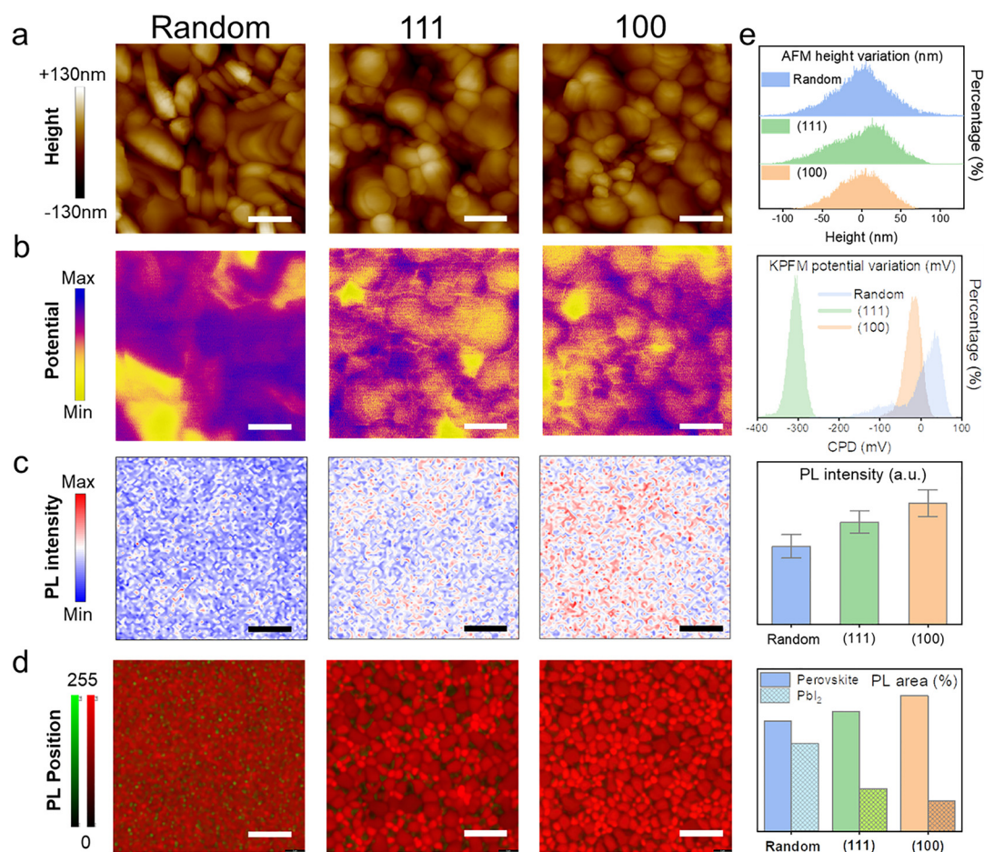
Fig. 4 Various perovskite films with different orientations visualized by AEM (scale bars, 1 μm) (a), KPFM (scale bars, 1 μm) (b), confocal PL-intensity mapping (scale bars, 20 μm) (c) and confocal PL-position mapping (scale bars, 5 μm) (d). (e) A visualization summary of the perovskite films by using the respective characteristic parameters of different visualization methods.
