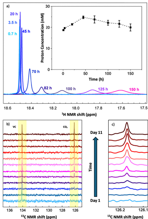
Fig. 3 Selected NMR spectra after electrochemical oxidation of the 1.3 M \text{LiClO}_4/\text{EC} electrolyte: (a) the ^1\text{H} shift of protons electrogenerated from a \text{LiClO}_4/\text{EC} electrolyte as a function of time after electrochemical oxidation. The inset shows the proton concentration calculated based on the peak area and calibrated with an external standard (10 mM VC). Standard deviation for each point is shown as an error bar. (b) ^{13}\text{C} NMR spectra (126–134 ppm) in the \text{LiClO}_4/\text{EC} electrolyte recorded each day from day 1 to day 11 highlighting VC and \text{CO}_2 generation. (c) Zoom-in of the \text{CO}_2 ^{13}\text{C} NMR signal change with time.
