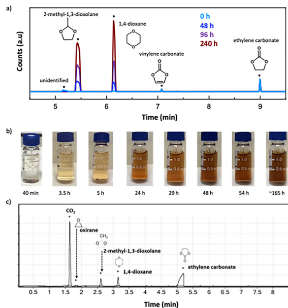
Fig. 4 (a) Detection of decomposition products with GC-MS using a Rxi-624Sil MS capillary column. 100 \mu\text{L} of the sample headspace was injected directly onto the column at various times elapsed after passing 45C of the charge through the electrolyte. (b) A change in colour was observed with time after the electrolyte was oxidized with 45C. (c) Detection of decomposition products with GC-MS. The headspace of a sample after passing 1.5C of the anodic charge through the electrolyte was analysed on day 7 using a dynamic headspace sampler and a DB-5MS capillary column.
