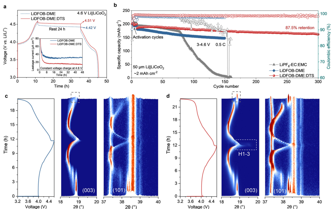
Fig. 6 The stability and structural evolution of \text{LiCoO}_2 charged to 4.6 V. (a) Voltage versus time curves display the self-discharge of \text{Li}||\text{LiCoO}_2 cells with different electrolytes. The inset shows the chronoamperometry test at 4.6 V at 1st cycle and a constant voltage charge process in \text{Li}||\text{LiCoO}_2 cells with different electrolytes. (b) Cycling performance of \text{Li}||\text{LiCoO}_2 cells with different electrolytes in the voltage range 3–4.6 V at 25 °C. (c) and (d) Voltage–capacity curve and the in situ XRD pattern of the \text{LiCoO}_2 electrode using (c) LiDFOB-DME and (d) LiDFOB-DME:DTS electrolytes during the initial cycle within a voltage range of 3–4.6 V at 0.1C.
